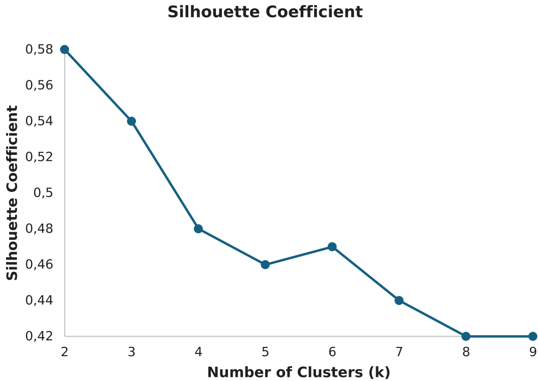
Graph 2. Quality of the obtained clusters using the silhouette coefficient
